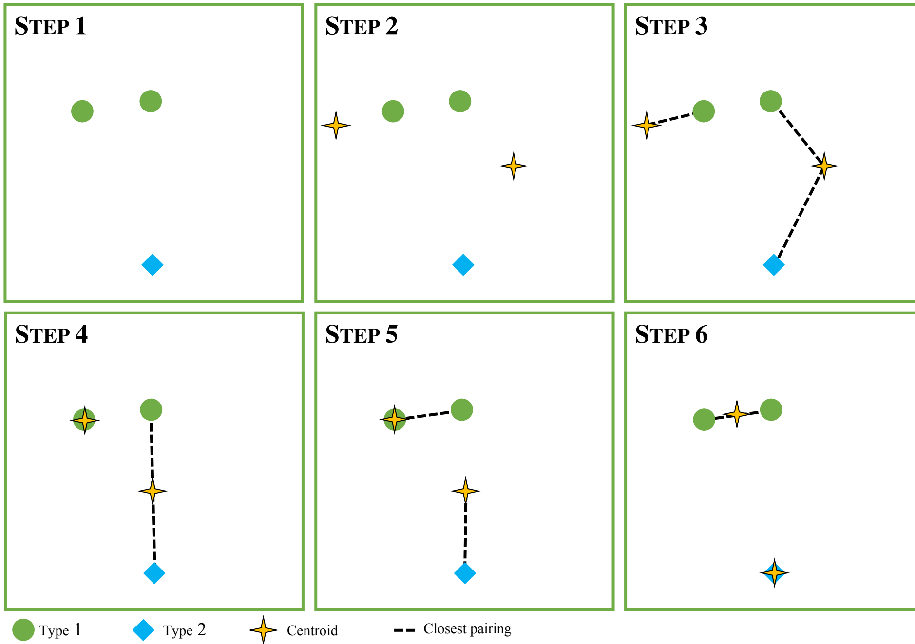
Figure S5. K-means Clustering Algorithm
